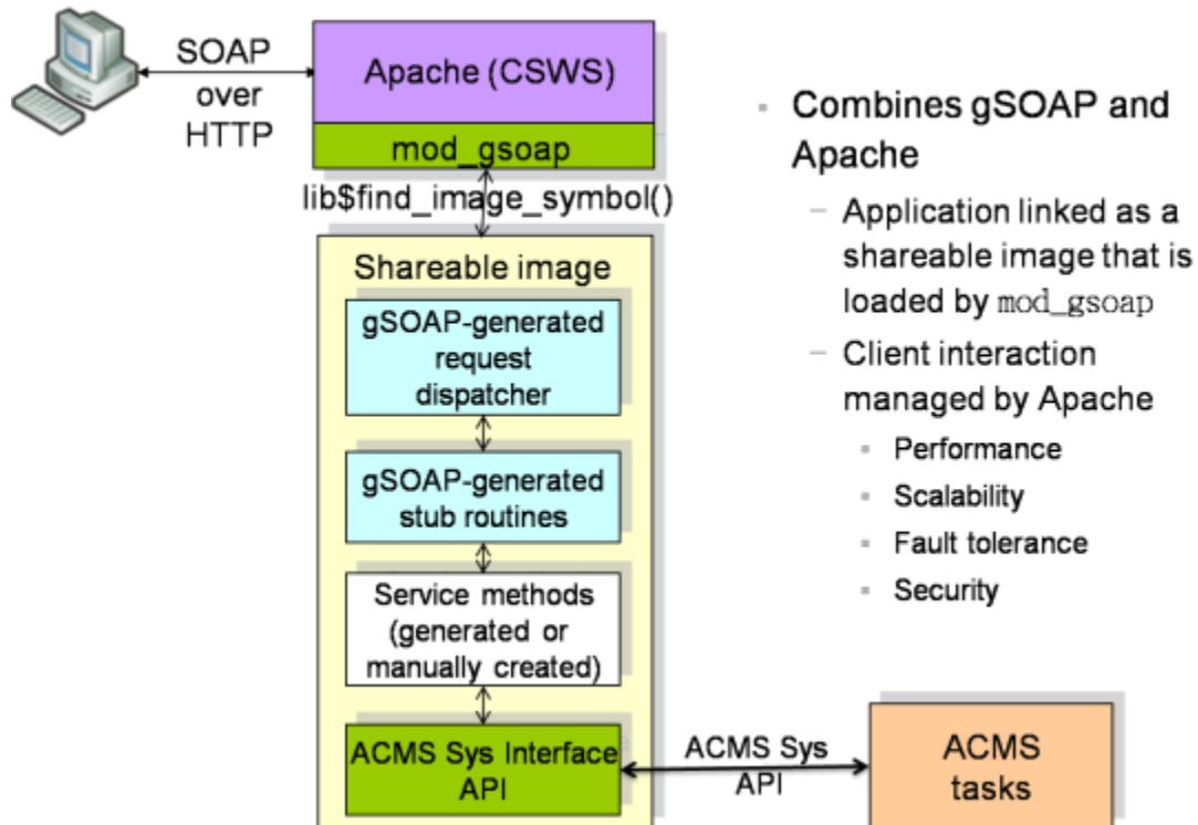
Figure 5 gSOAP with Apache and mod_gsoap
