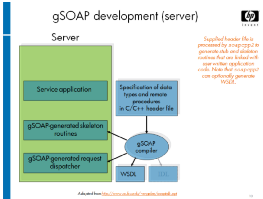
Figure 2 gSOAP Development, Server
