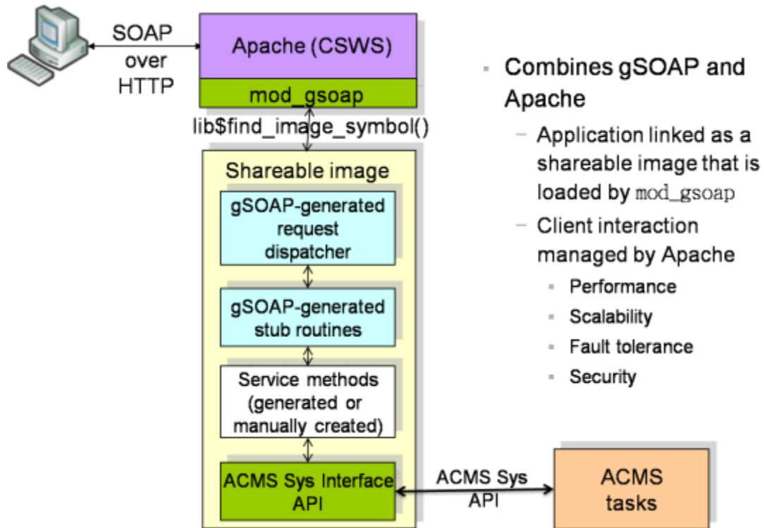
Figure 4 gSOAP with ACMS and mod_apache
